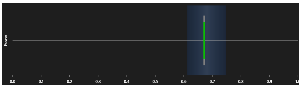
Echo Detected at Member Diameter
